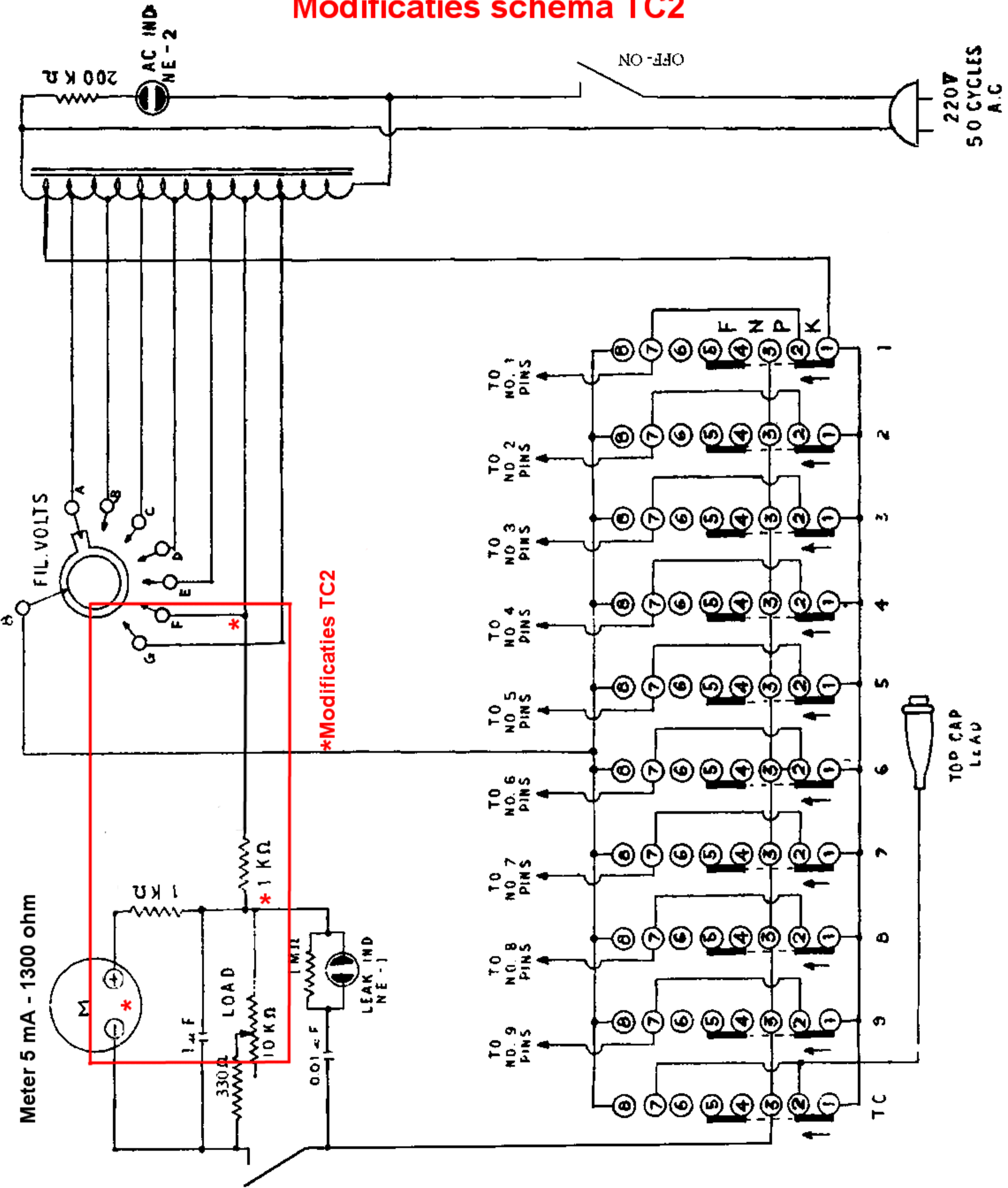
SCHEMATIC DIAGRAM
